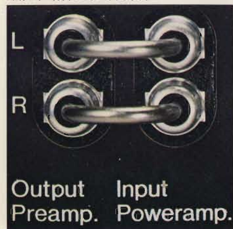
Separate preamplifier outputs and power amplifier inputs permit interfacing such accessories as equalizers or reverberation amplifiers. The newly-designed preamplifier is capable of an output of up to 5 volts with less than 0.1% distortion.
