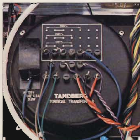
Tandberg's shielded toroidal transformer, prevents stray fields that can cause hum.
