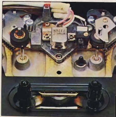
Dual-capstan closed-loop drive system in combination with 3 motors, a Tandberg innovation, ensures smooth, gentle tape flow across the head, where it matters most.
