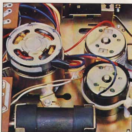
The three specially-designed motors eliminate the need for mechanical clutches that will wear out and degrade performance.
