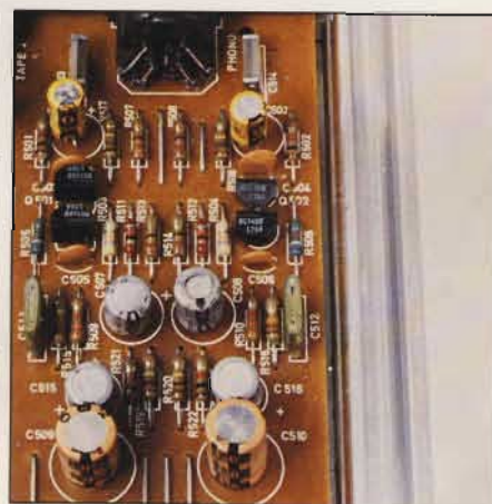
Phono signals are connected directly to a separate RIAA equalizer circuit.
